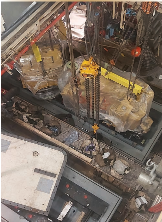
Figure 5. A new engine and generator are positioned on the machinery raft.
