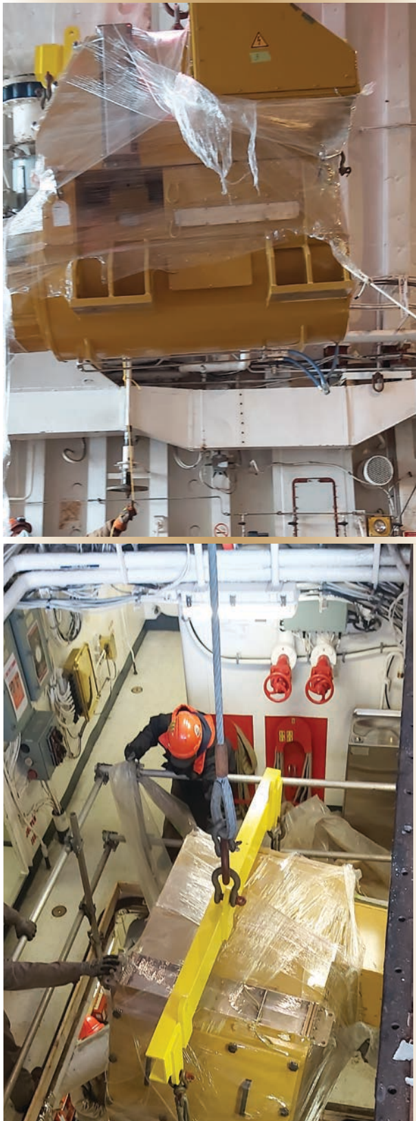
Figure 3a and b. A new Hitzinger generator is moved through the ship's hangar, and lowered into the AAMR.
